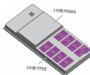
2-color molding product (PMMA + TPEE)
