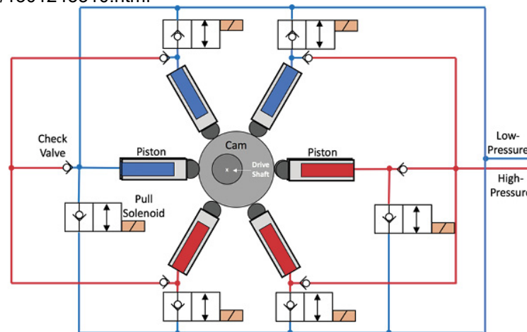
Fig. 3 Solenoids Energized, Full Flow
